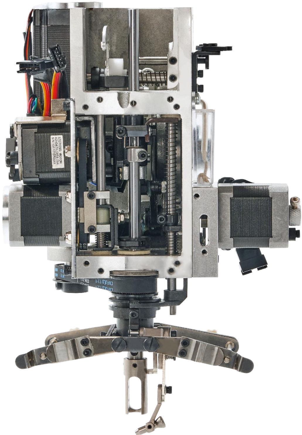
Taping device PDX11A
